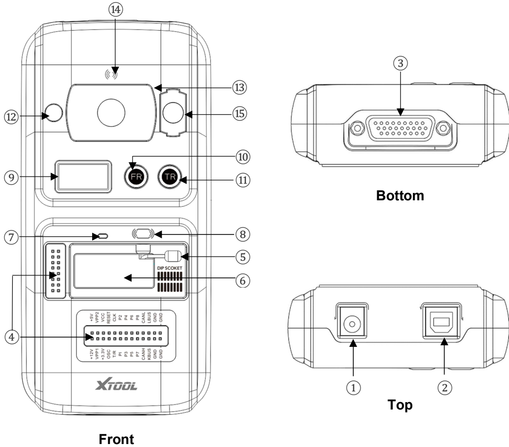
Fig 1-7 KC501 Exposed View
